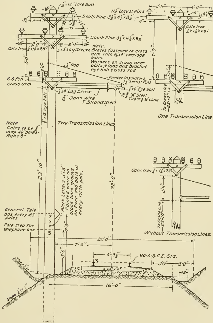
Fig. 172. Diagram of Construction of Single-Track Interurban Trolley Road
